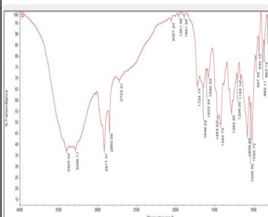
Figure 7: FTIR spectra of atropine sulfate with sodium starch glycolate based formula.
