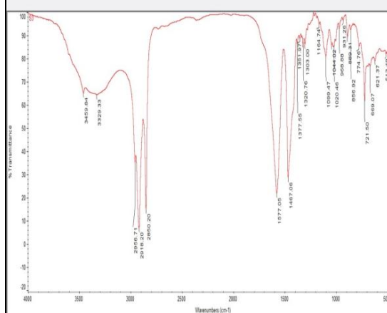
Figure 6: FTIR spectra of atropine sulfate
