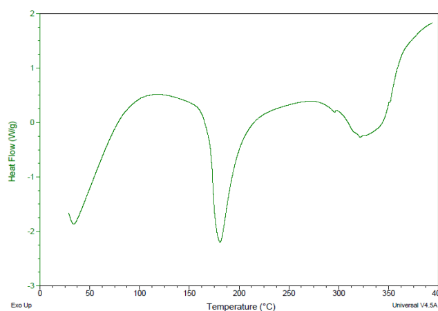
Figure 4: DSC thermogram of atropine sulfate and physical mixture of crospovidone based formula
