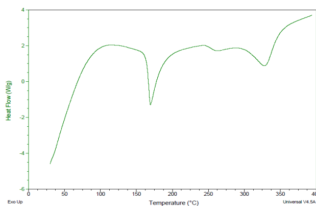
Figure 3: DSC thermogram of atropine sulfate
