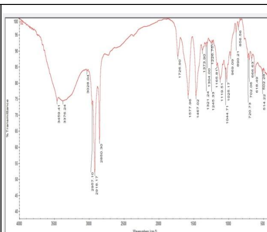
Figure 7: FTIR spectra of atropine sulfate with sodium starch glycolate based formula.
