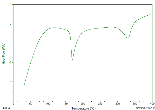
Figure 2: DSC thermogram of atropine sulfate and physical mixture of crosscarmellose based formula
